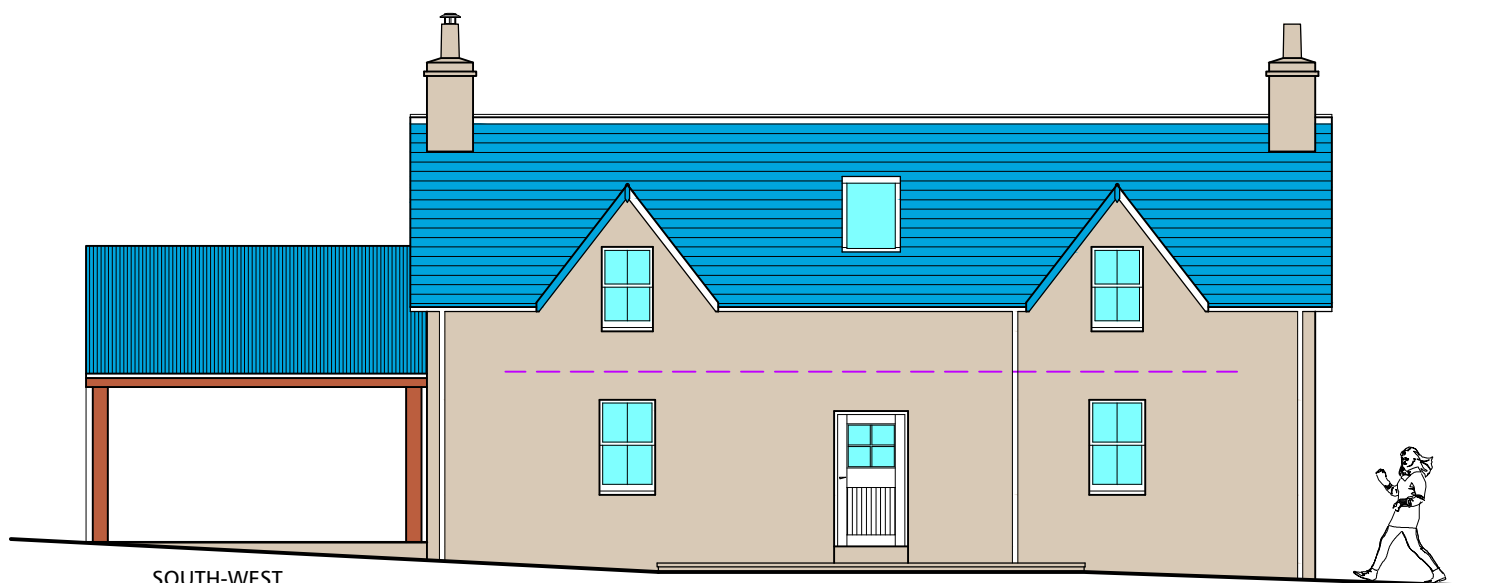
SOUTH-WEST ELEVATION
